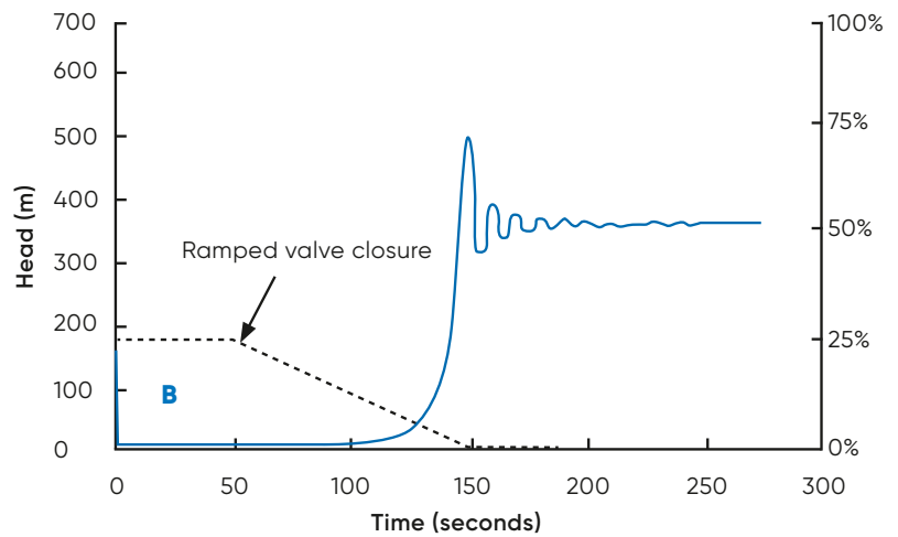
A Pressure response to valve closure of downhill pipeline. B Pressure response to ramped valve closure of downhill pipeline.
