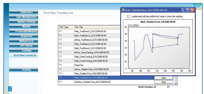
A The view from the simulator is identical to the actual DCS screen.
